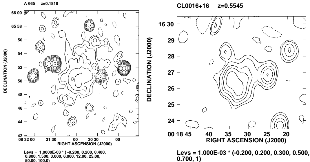
Figure 1: Left panel: Image of the giant radio halo detected at the center of A 665. The HPBW is 42'' \times 52'' (RA \times DEC). Right panel: Image of the radio halo present in the central region of the distant cluster CL 0016+16. The HPBW is 45'' \times 60'' (RA \times DEC).
